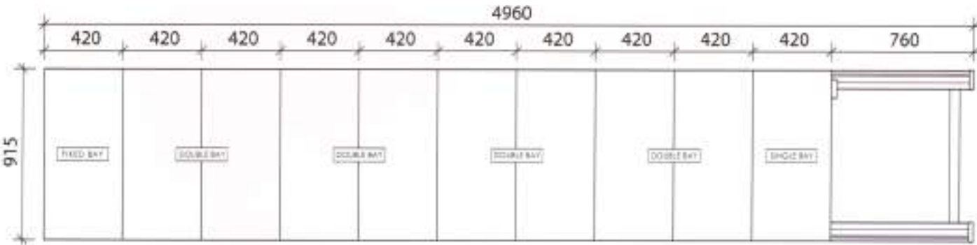
10 x 1 bay depth hand push mobile compactor
