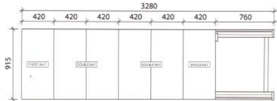
6 x 1 bay depth hand push mobile compactor
