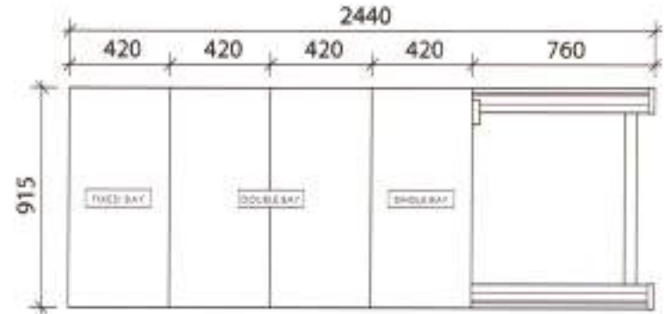
4 x 1 bay depth hand push mobile compactor
