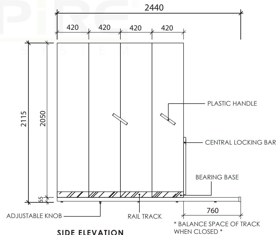
SIDE ELEVATION
