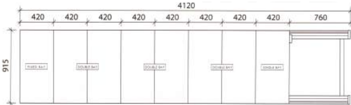
8 x 1 bay depth hand push mobile compactor
